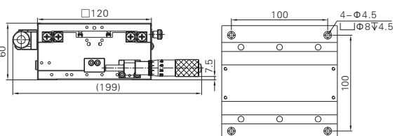
XYC120
