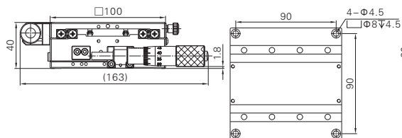
XYC100
